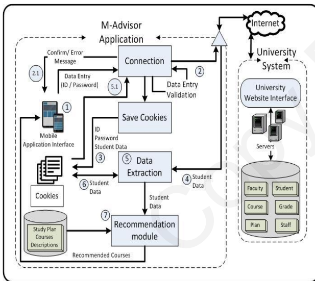
Figure 1: The architecture of m-advisor
