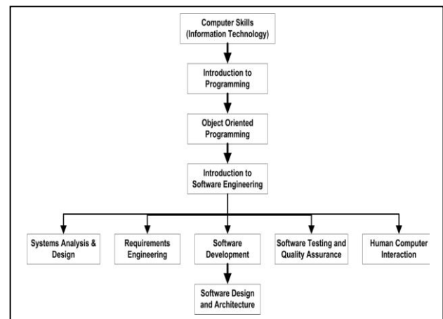
Figure 2: The Prerequisite structure of the compulsory department requirements (BSc degree in Software Engineering)
