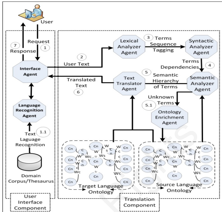
Fig 1. The Semantic Multi-agent Architecture for Multilingual MT
